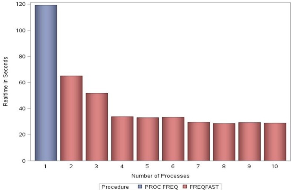
Figure 4. Realtime Comparison of FREQ Procedure and FREQFAST with Incrementing Parallel Processes
