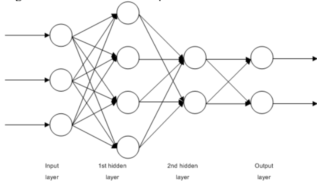
Figure 8. Architecture of Deep Neural Networks
