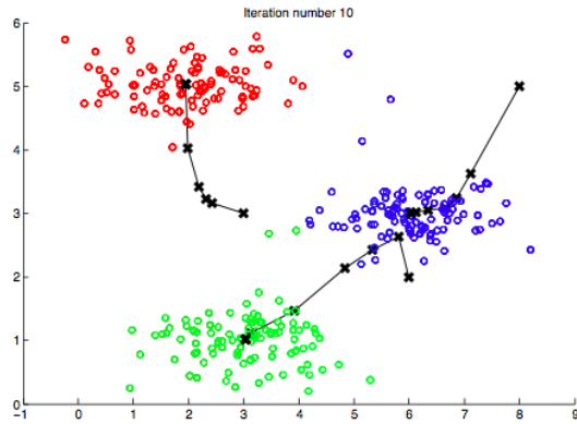
Figure 6. Clustering algorithm
