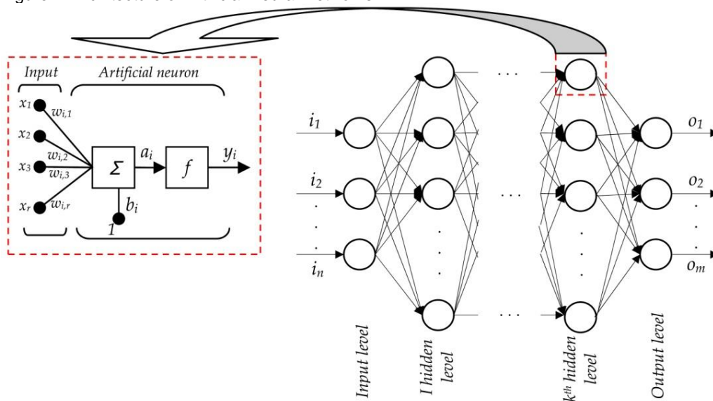
Figure 7. Architecture of Artificial Neural Networks
